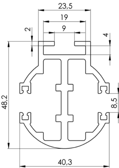
Double-Sided Round Guiding Channel P 017/7 (7-302155)
