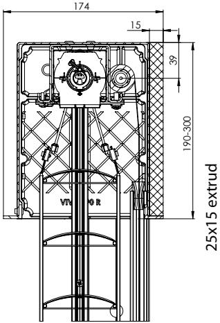
Cut of under plaster self-supporting blind VIVA (ready for polystyrene on front part+ polystyren on back part). Heat insulation behind the box must not exceed 15 mm regardless of the box offset! Extruded
