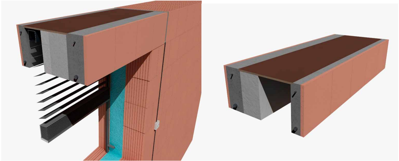
The blind is fitted in the lintel in clamps anchored in the upper water-proof plywood board.
