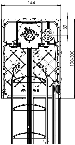
Cross section fo the visible self-supporting blind Viva
