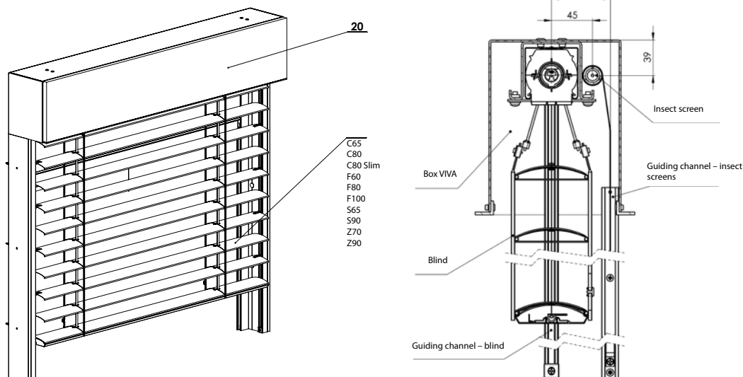
SELF-SUPPORTING BLIND VIVA 2-01010-0000-B
