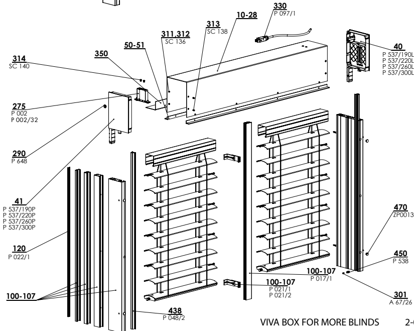
VIVA BOX FOR MORE BLINDS
