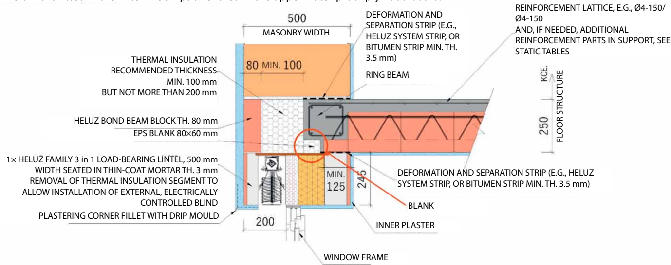
The blind is fitted in the lintel in clamps anchored in the upper water-proof plywood board.
